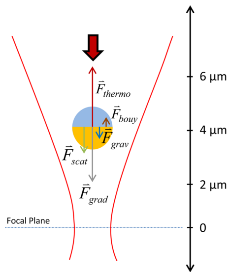
Figure 3. Force diagram of the microelevator system.
